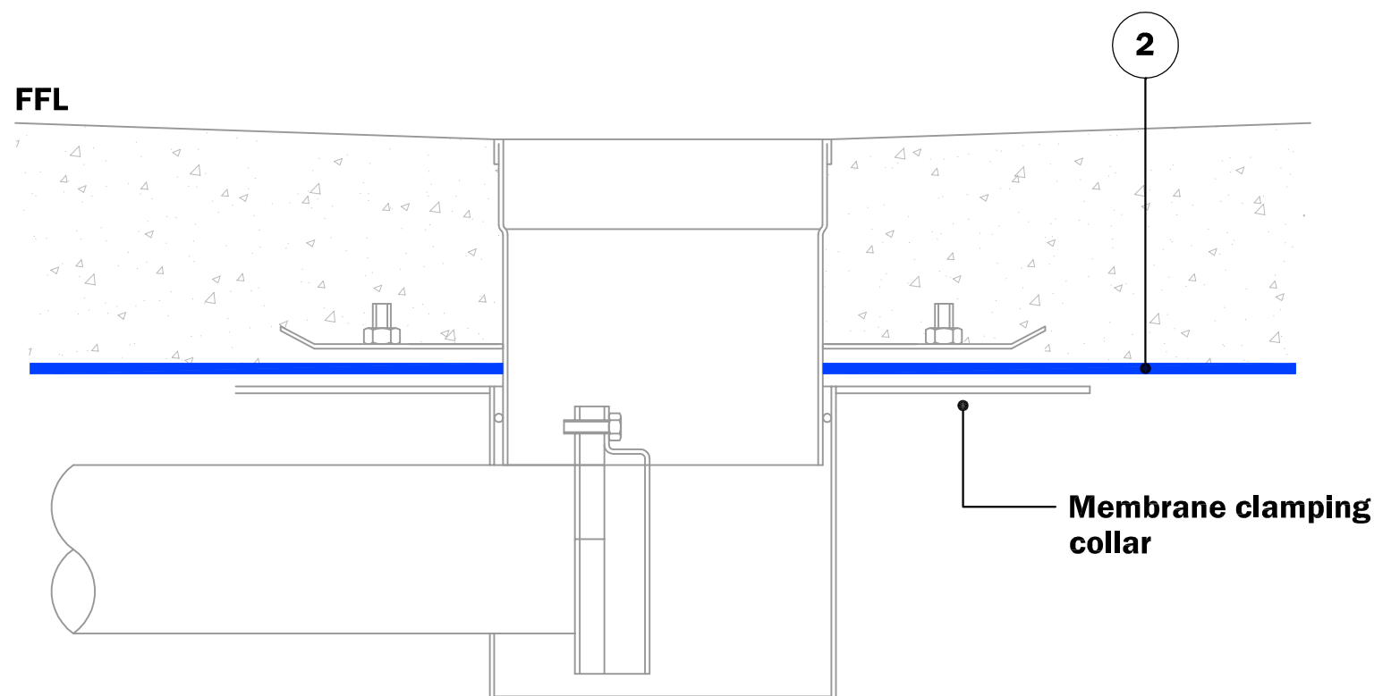
Generic Floor Gully
