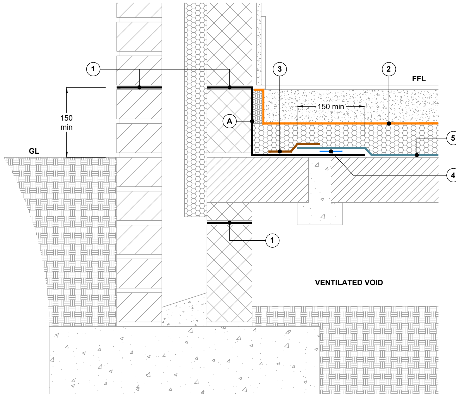
Section View
