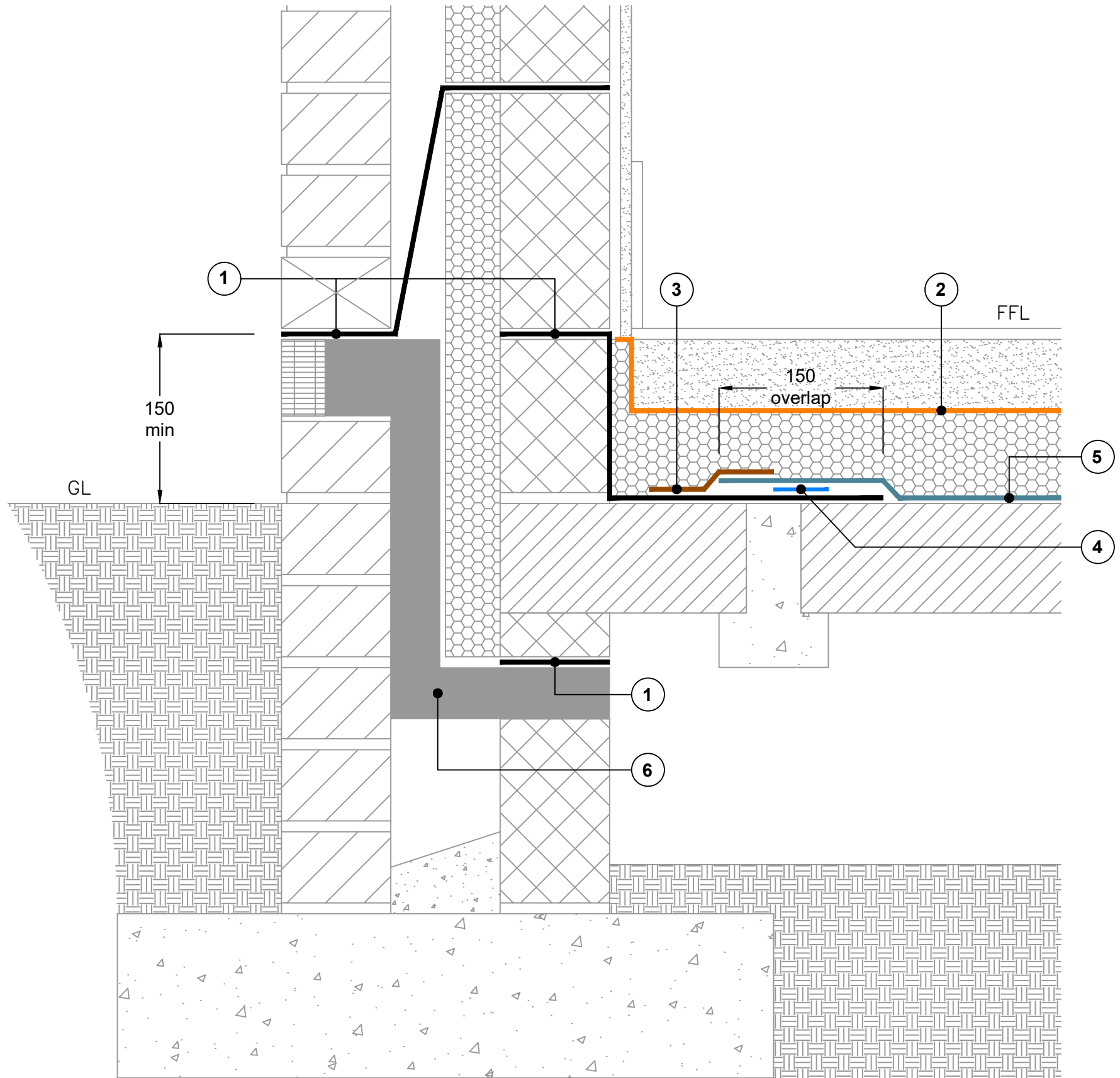
Section View
