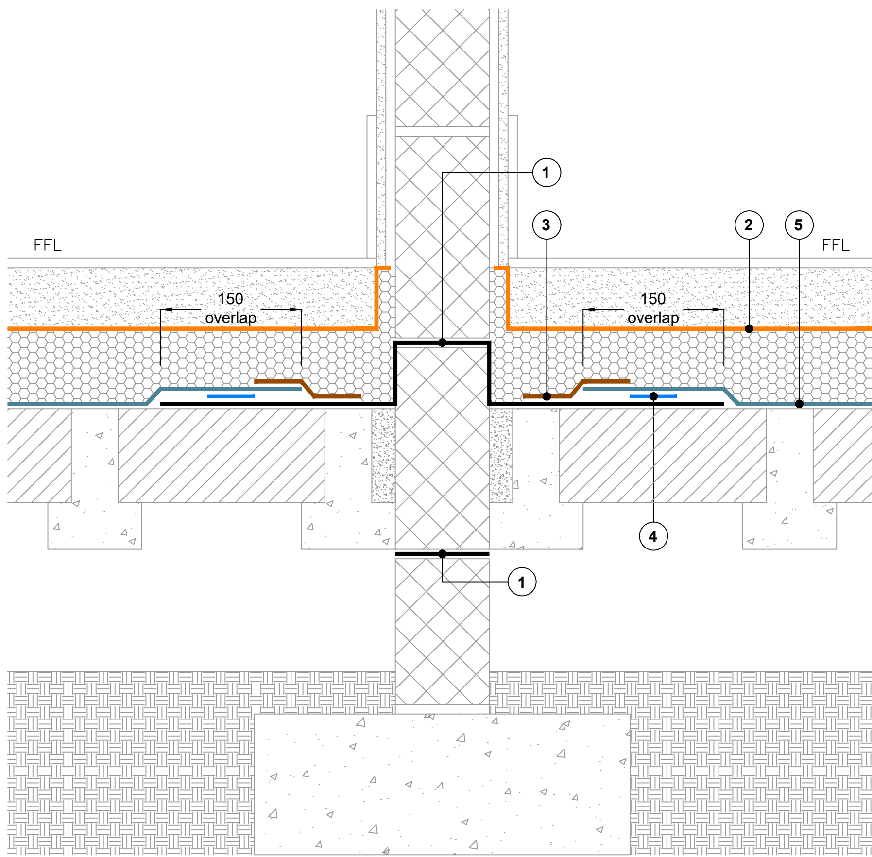
Section View
