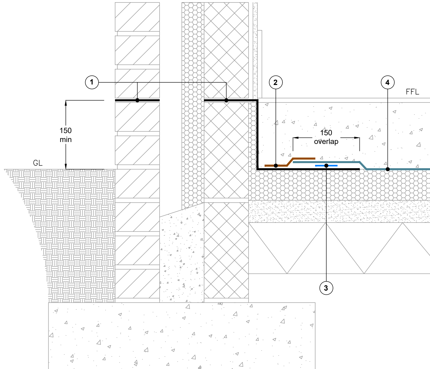
Section View
