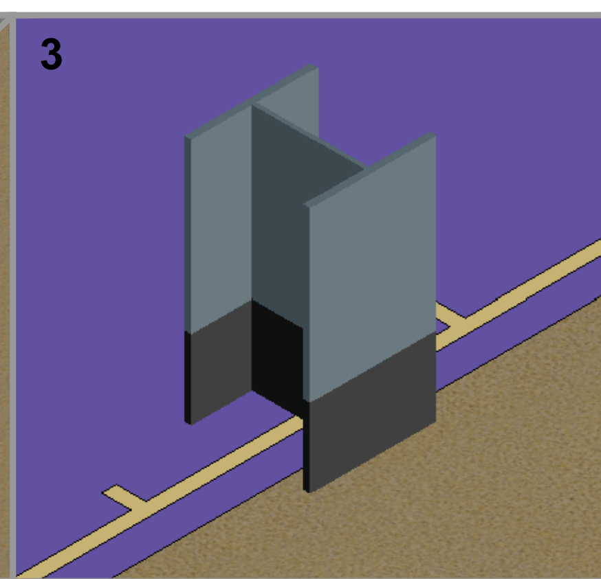
3 Cut and install Visqueen Ultimate RadonBlok 600 around column. Apply Visqueen Ultimate RadonBlok Double Sided Tape.
