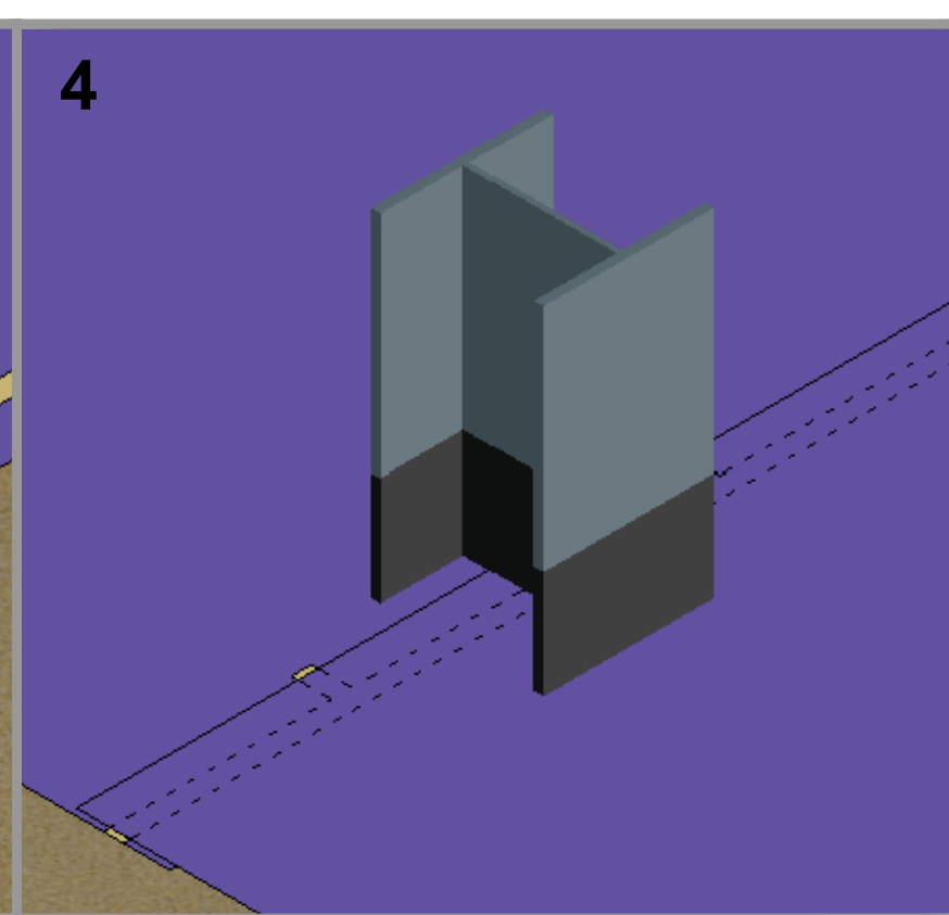
4 Cut and install adjacent membrane around column, bonding to Visqueen Ultimate RadonBlok Double Sided Tape.
